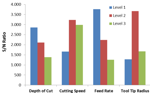
Figure 4. S/N response for surface roughness values
