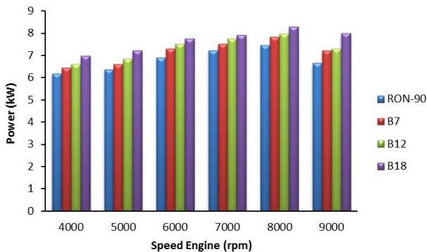
1 Figure 3. Comparison of output power to engine speed
