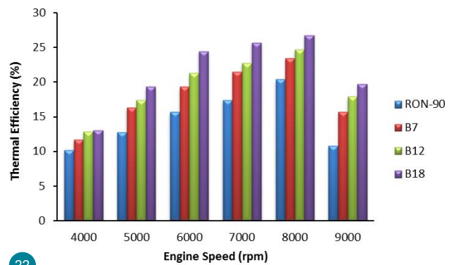
Figure 7. Comparison of thermal efficiency to engine speed
