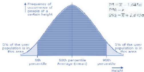
Gambar 3. DistribusiNormal
