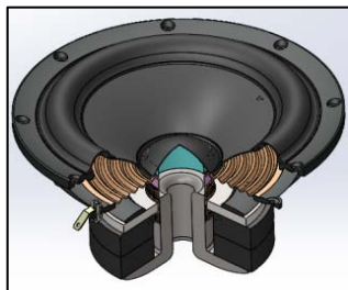
Gambar 1 Assembly Speaker
