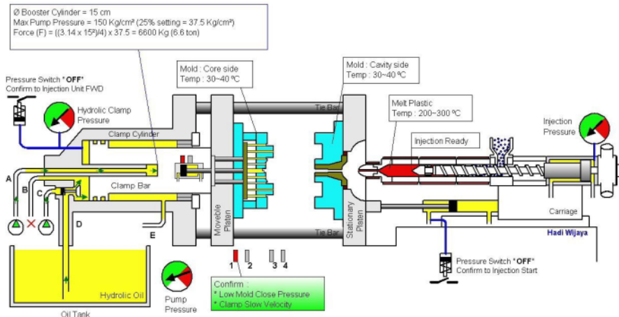
Gambar 2. Machine Injection Plastic
